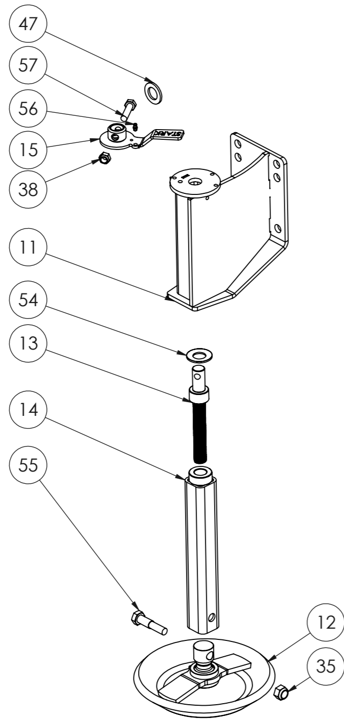
DETAIL A SCALE 2 : 15
