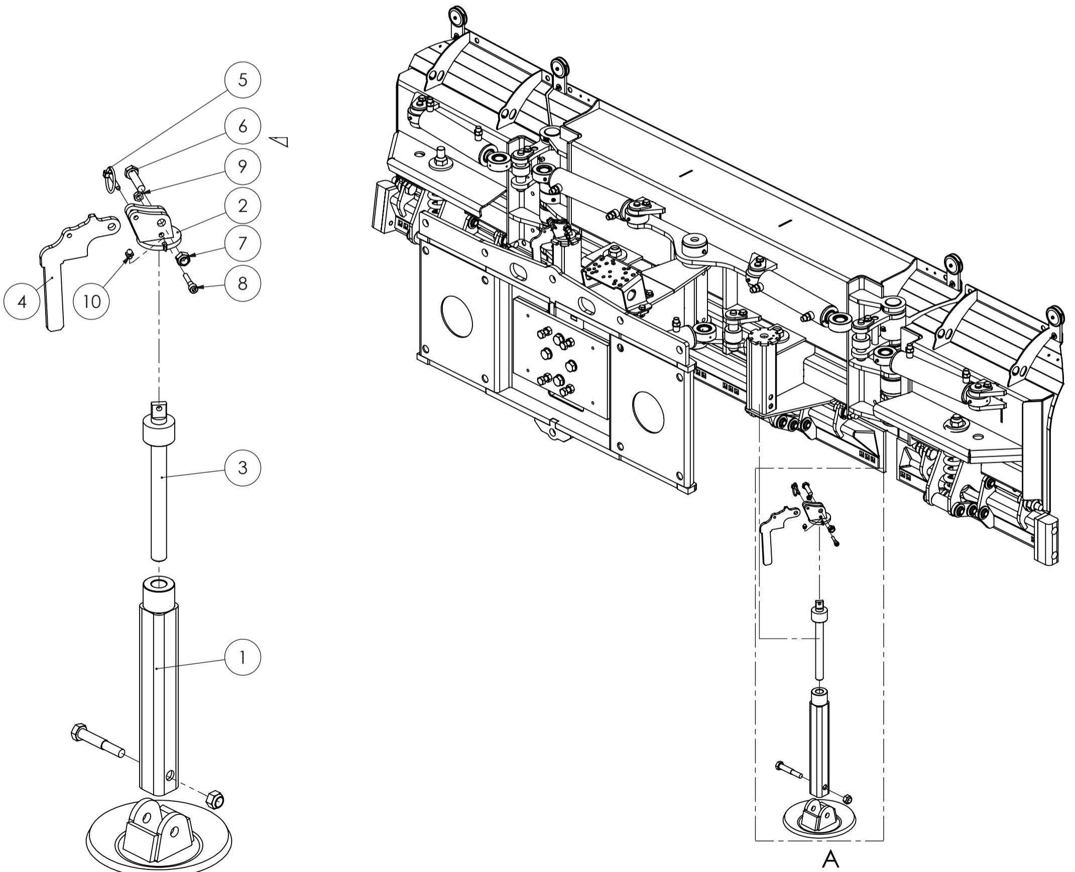
DETAIL A SCALE 1 : 6
